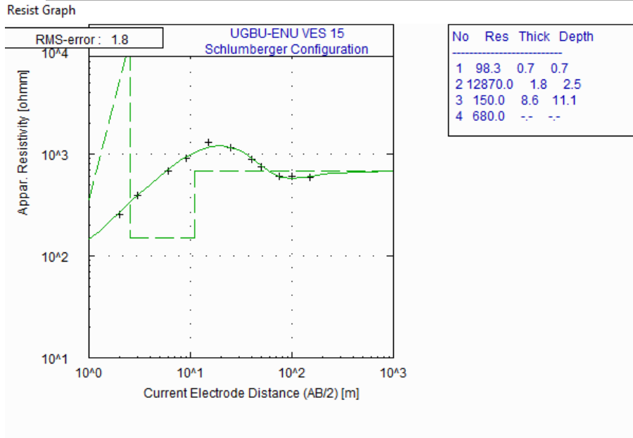
Fig. 17: Winresistivity plots of VES I5 Location in Awka North LGA
