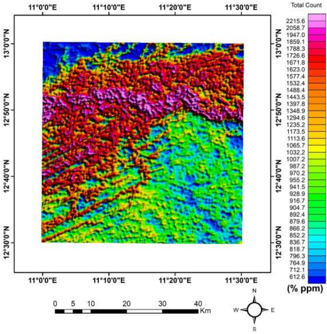
Figure 12: TC Map of the Study Area
