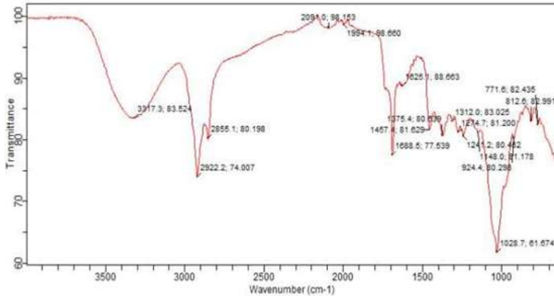
Figure 9: Fourier Transform Infrared (FTIR) spectra of Centella asiatica (Gotu kola)
