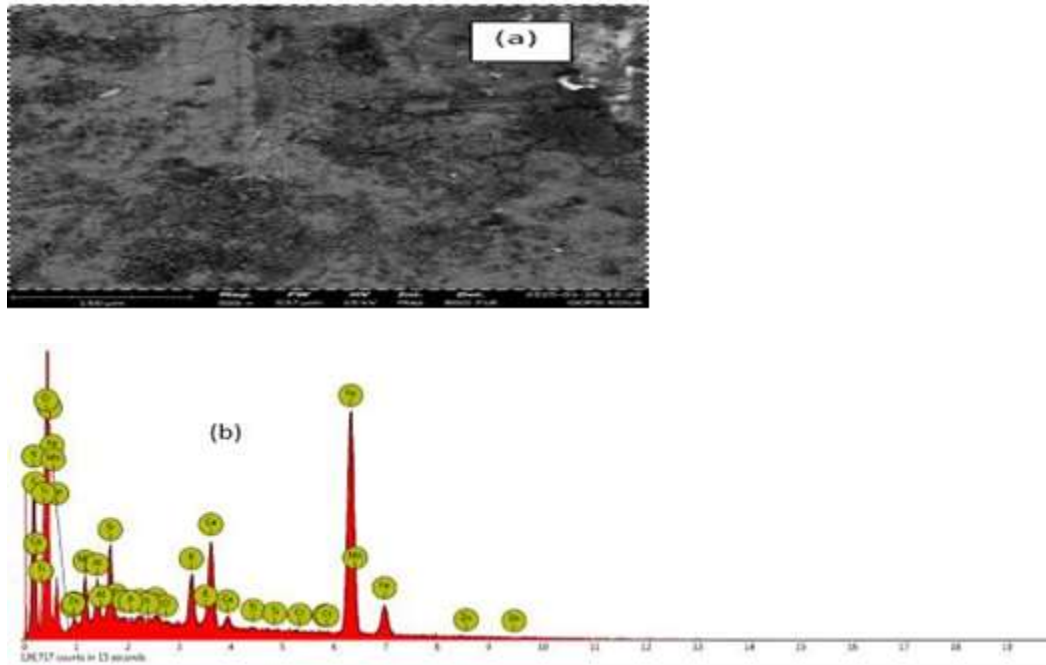
Figure 11: (a) SEM image and (b) EDS spectrum of mild steel with Centella asiatica extracts
